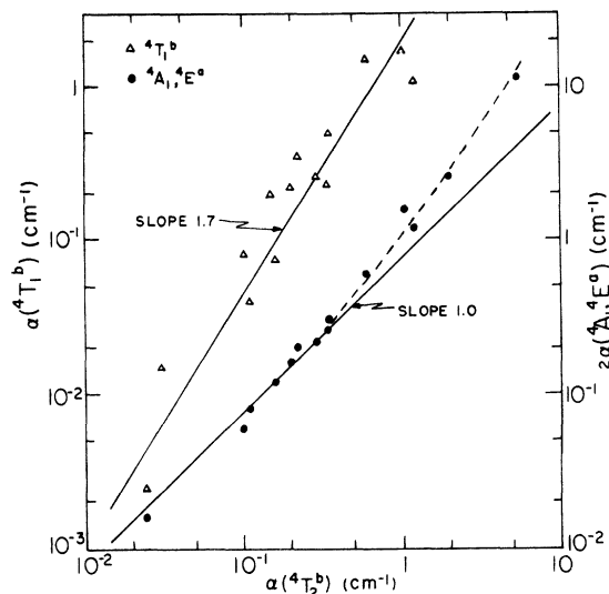
FIG. 6. Dependence of \alpha(^4A_1, ^4E^a) and \alpha(E^b) on concentration at room temperature. [ \alpha(^4T_2^b) is proportional to the concentration.] The quantity \alpha = l^{-1} \log_{10}(I_0/I) .
